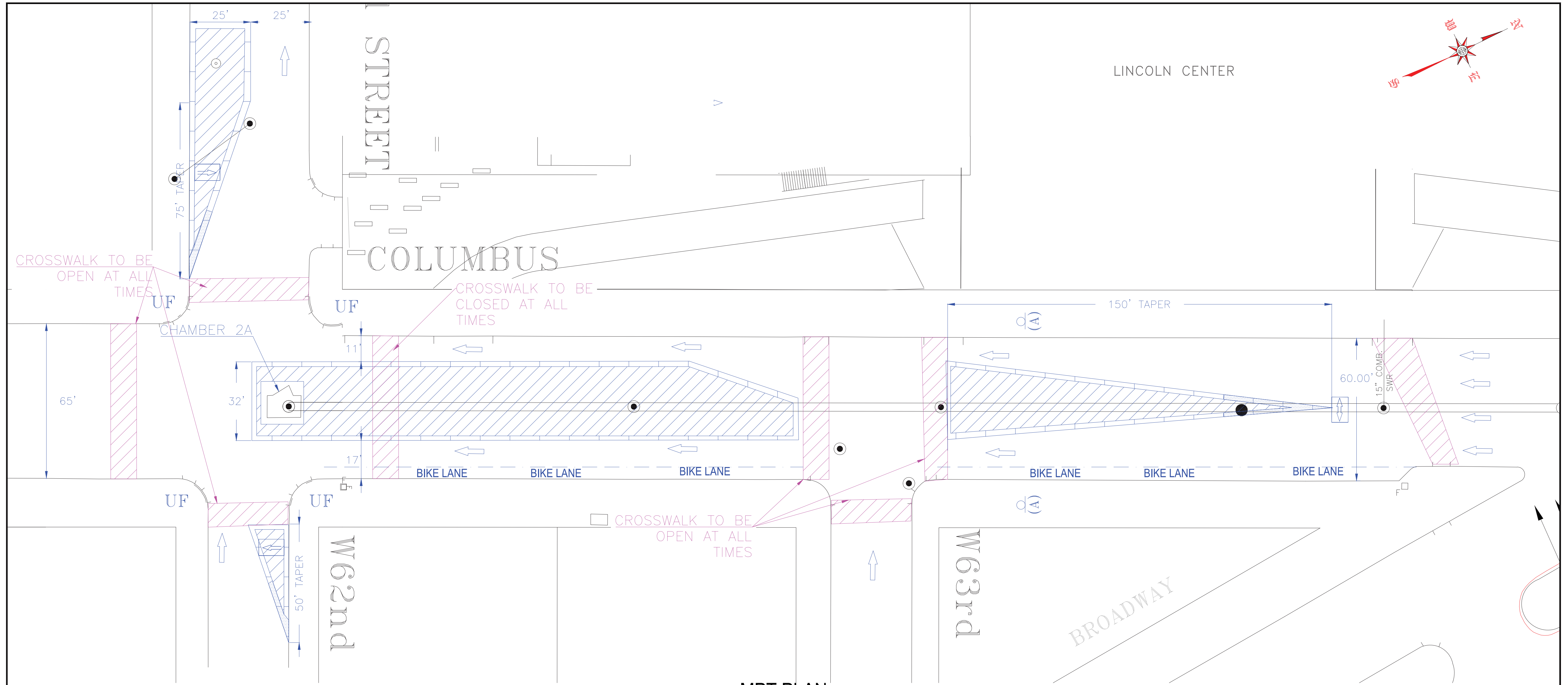
MPT PLAN MPT CONFIGURATION ON COLUMBUS FOR SEWER WORK AND CHAMBER 2A
